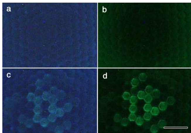
Figure 7. Fluorescence microscopic photographs of the eyes of female ( a, b ) and male ( c, d ) P. rapae crucivora , at the level of the corneal facet lenses, under UV ( a, c ) and violet ( b, d ) excitation. Whereas the fluorescence in female eyes is more or less homogeneous and faint, that of type II ommatidia in male eyes is distinct [for the relationship of the fluorescence and the ommatidial types, see Qiu et al. (2002)]. Scale bar, 50 \mu m.
