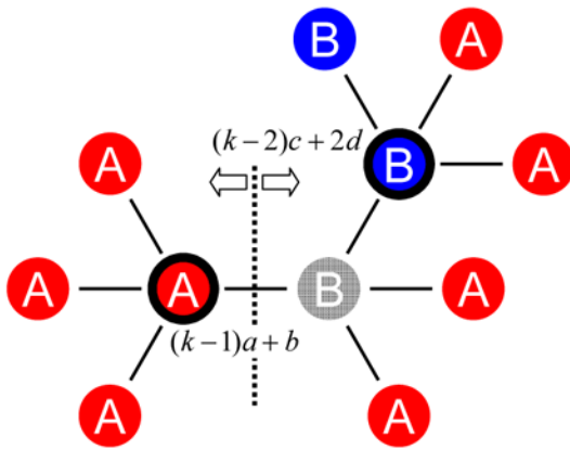
Figure 4. A simple way to reproduce the ESS condition for DB updating. The focal boundary is drawn in a dotted line. Those who are involved in the movement of the boundary are marked with circles. Payoffs are shown next to players. Top: when the A-player at the boundary dies. Bottom: when the B-player at the boundary dies.
