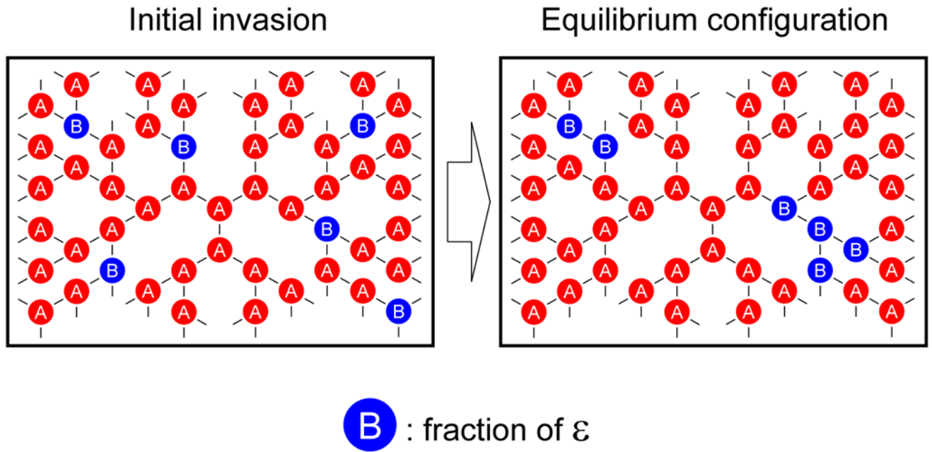
Figure 1. Local configuration of rare B mutants quickly equilibrates into clusters, without changing the total number of initial B players.
