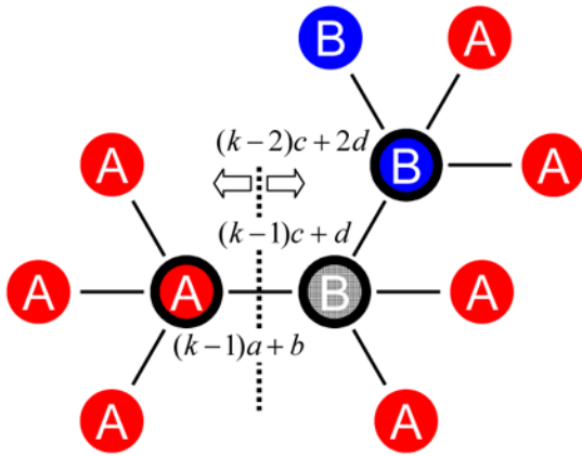
Figure 5. A simple way to reproduce the ESS condition for IM updating. The focal boundary is drawn in a dotted line. Those who are involved in the movement of the boundary are marked with circles. Top: when the A-player at the boundary dies. Bottom: when the B-player at the boundary dies.
