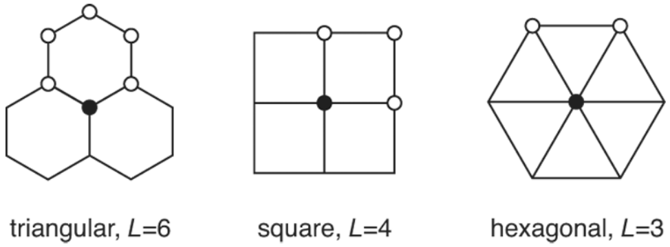
Figure 8. The length of the minimal loop, L , is shown for triangular, square, and hexagonal lattices, respectively.
