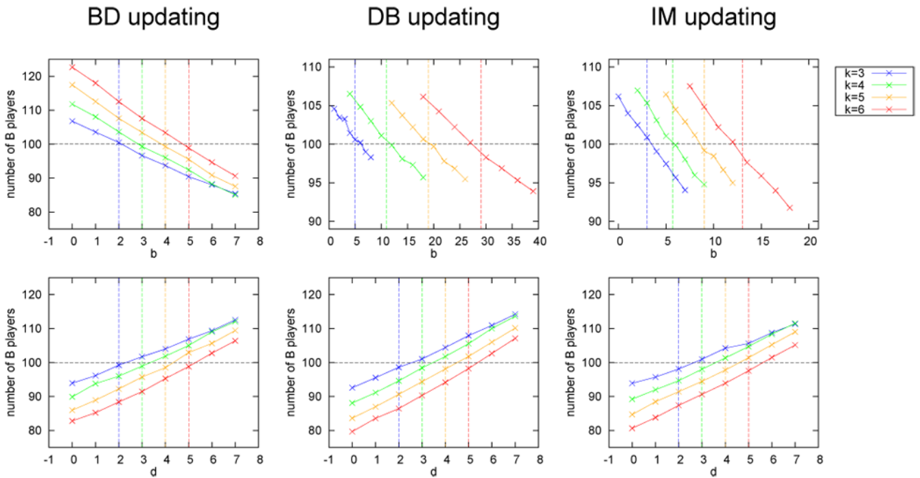
Figure 6. Computer simulation results for random regular graphs of degrees k = 3 (blue), k = 4 (green), k = 5 (orange), and k = 6 (red). Each column of panels in the figure represents one of the three update rules, BD (panels in the left), DB (panels in the center), and IM (panels in the right). In the top three panels, we study the parameter (a, b, c, d) = (0, b, 1, 0) so b is the only free parameter, which is shown in each x-axis. In the bottom three, we study the parameters (a, b, c, d) = (1, 0, 0, d) , so d is the free parameter shown in each x-axis. The y-axis of each panel represents the average number of B players after 5 generations over 10^4 runs. In each small panel, the initial number of B players, that is n_B = 100 , is shown by the black horizontal dotted line. Thus, the number of B players after 5 generation being below this threshold, n_B = 100 , implies that strategy A is an ESS. For each degree k , simulation results are plotted in a corresponding color with 'x'-symbols. A colored vertical dotted line represents the theoretical prediction, eqs.(22–23). The simulation data show a perfect agreement with theoretical predictions if both data plots and a vertical dotted line in the same color intersect with the black horizontal dotted line exactly at the same point.
