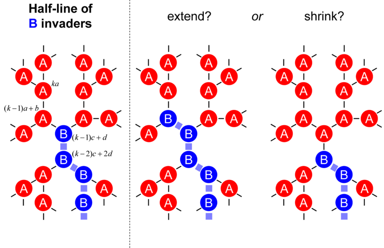
Figure 2. A schematic drawing where rare B -mutants invade the population of A -players in a half-line shape. The number shown next to player is his payoff. When the half-life is more likely to shrink than to extend, strategy A is an ESS.
